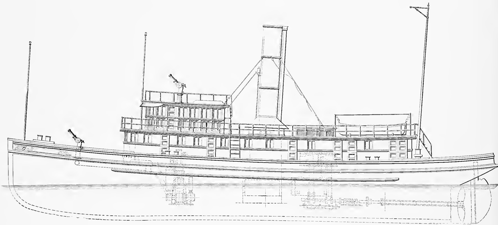
THE NEW WOODEN FIRE BOAT FOR THE CITY OF BOSTON.—Built by John M. Brooks, East Boston, Mass.
